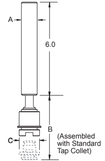
Straight Shank
