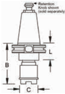
CAT40 Shank
